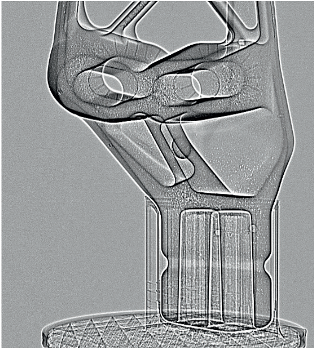
Side mirror x-ray image with optimized settings for manual 2D inspection.
